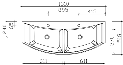
1310 mm BMD033M13101
